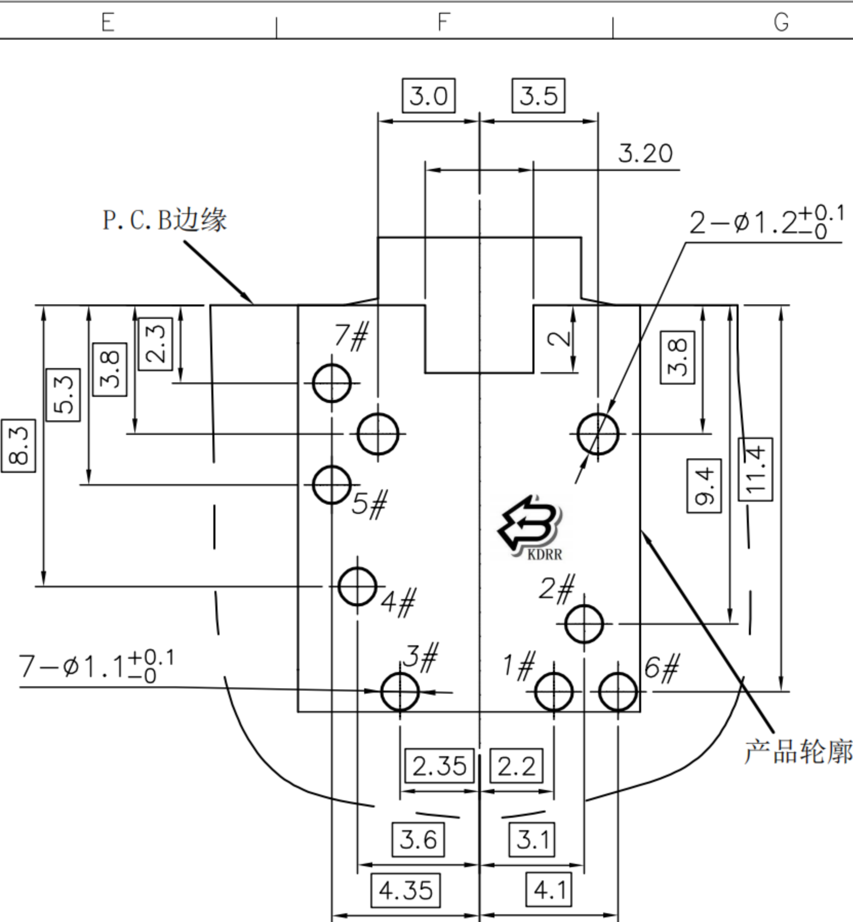
P.C.B LAYOUT TOP VIEW
